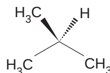
methylpropane
