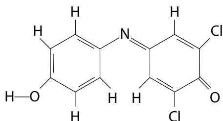
Oxidised DCPIP
