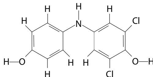
Reduced DCPIP
