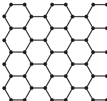
graphene
